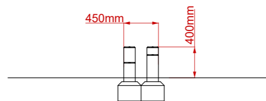
End View
